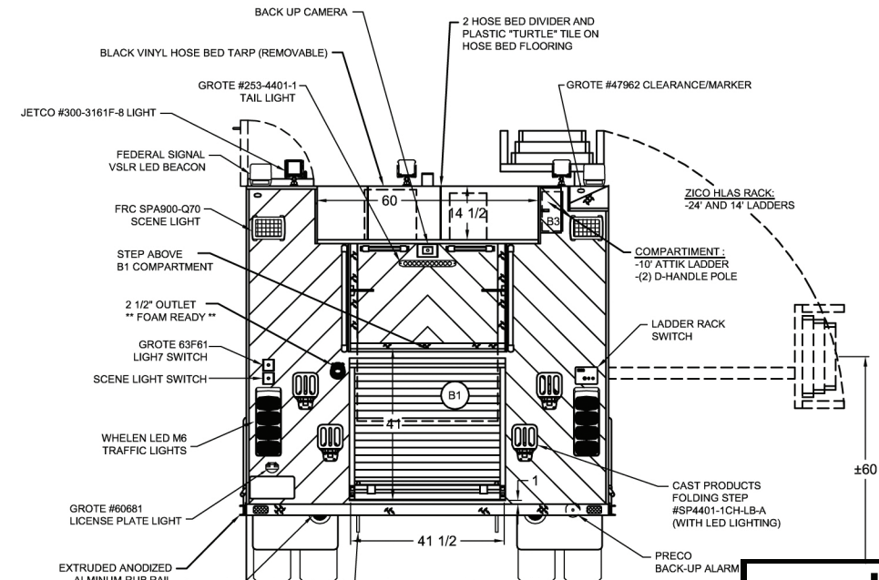
REAR VIEW
