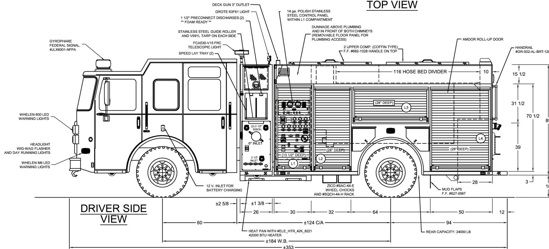
PRELIMINARY LAYOUT DELUXE 750 (DSD PUMP NARROW PANEL)
