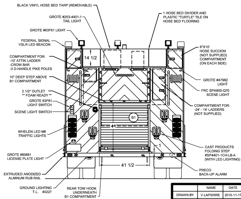
REAR VIEW
