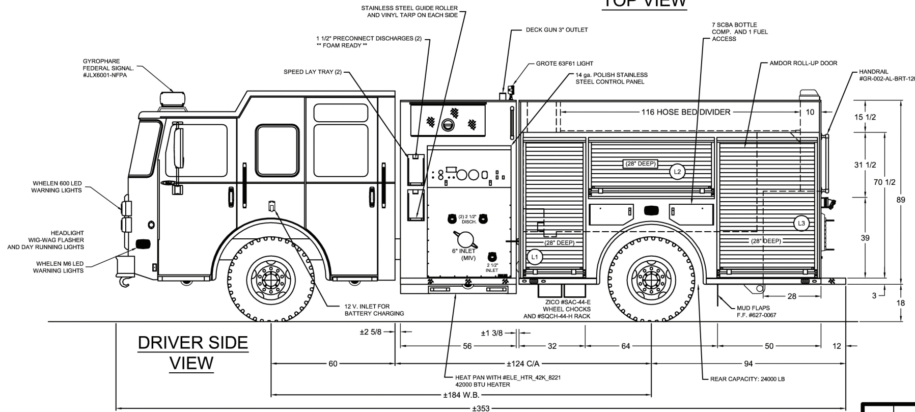
PRELIMINARY LAYOUT INTERMEDIATE 750 (QPUMP STANDARD PANEL)
