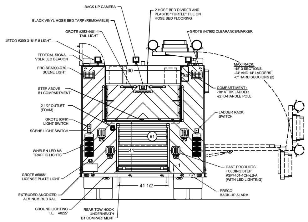
REAR VIEW
